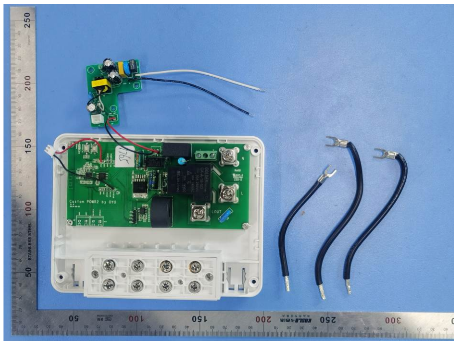
Figure 8 Internal View
