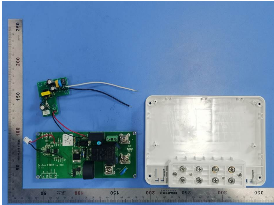
Figure 9 Internal View
