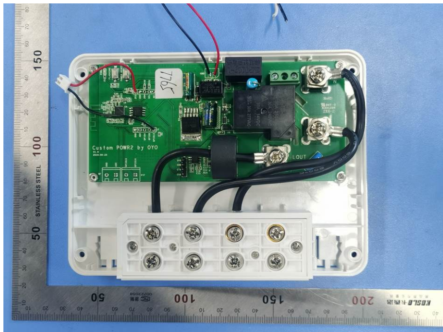
Figure 7 Internal View
