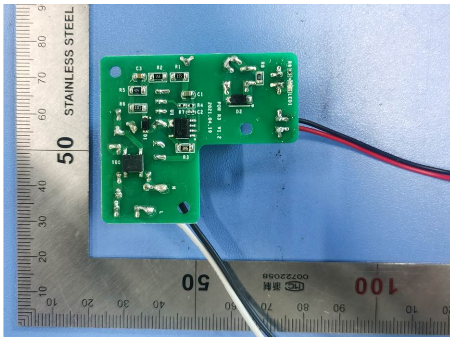
Figure 6 Internal View
